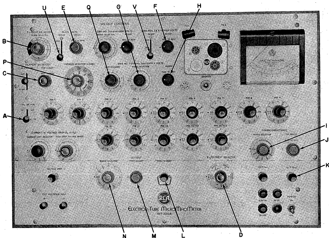
Figure 2. Controls used in testing a 6AG7 Power Pentode
